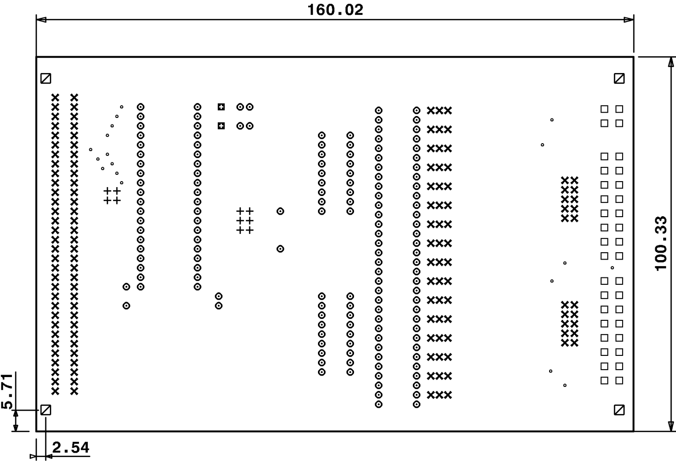
Drill Report : Layer E509023-60
