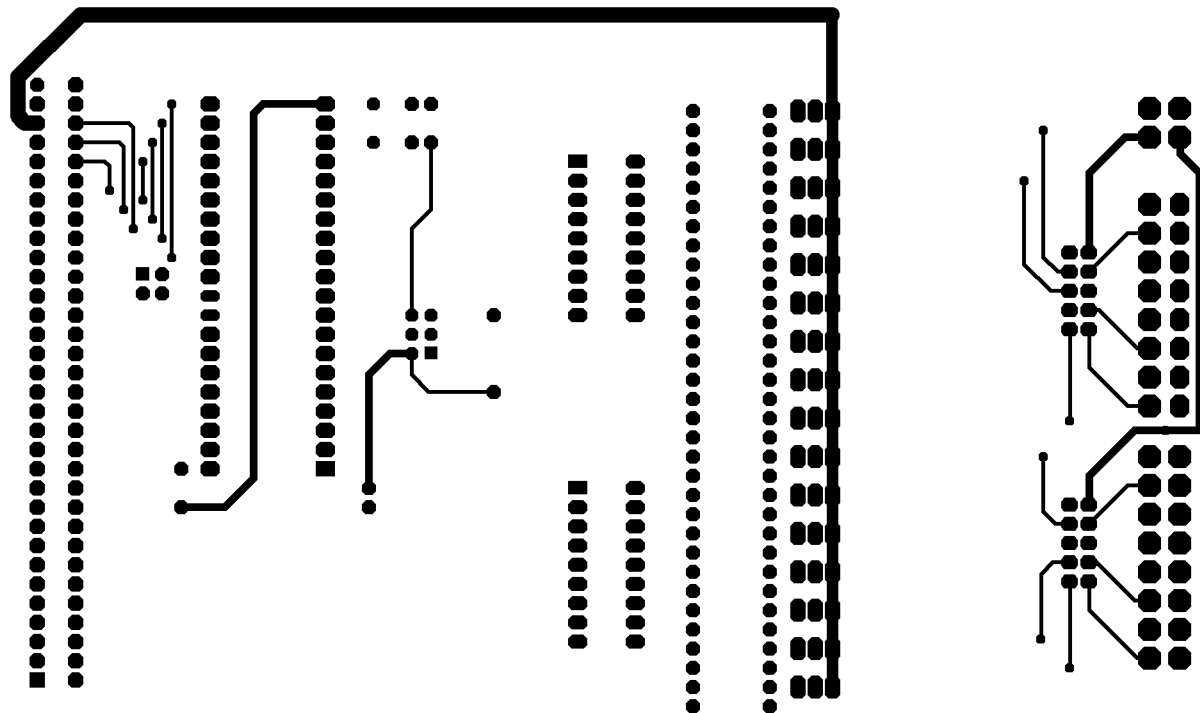
E509023 TOP layer Image (topview)
