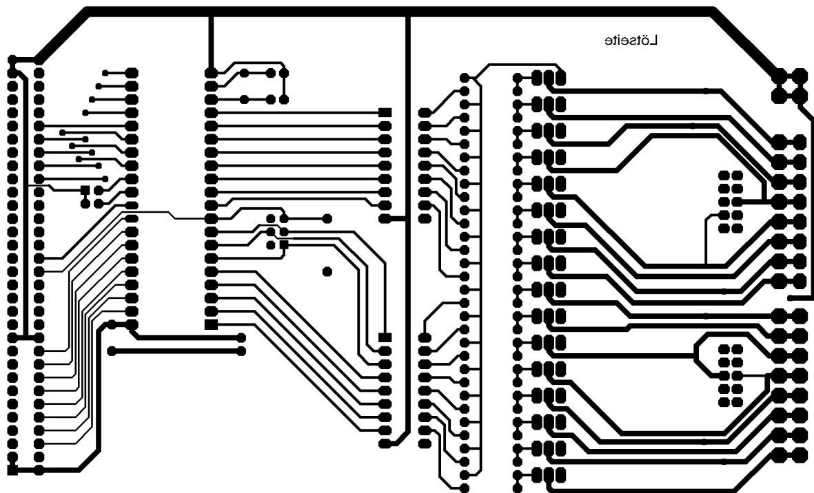
E509023 BOTTOM layer Image (topview)
