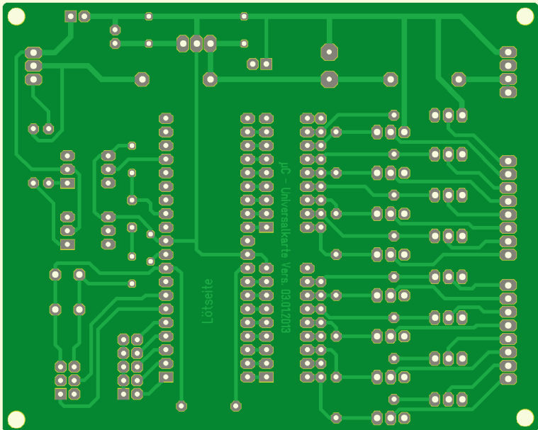
E516969 PCB view BOTTOM (bottomview)
