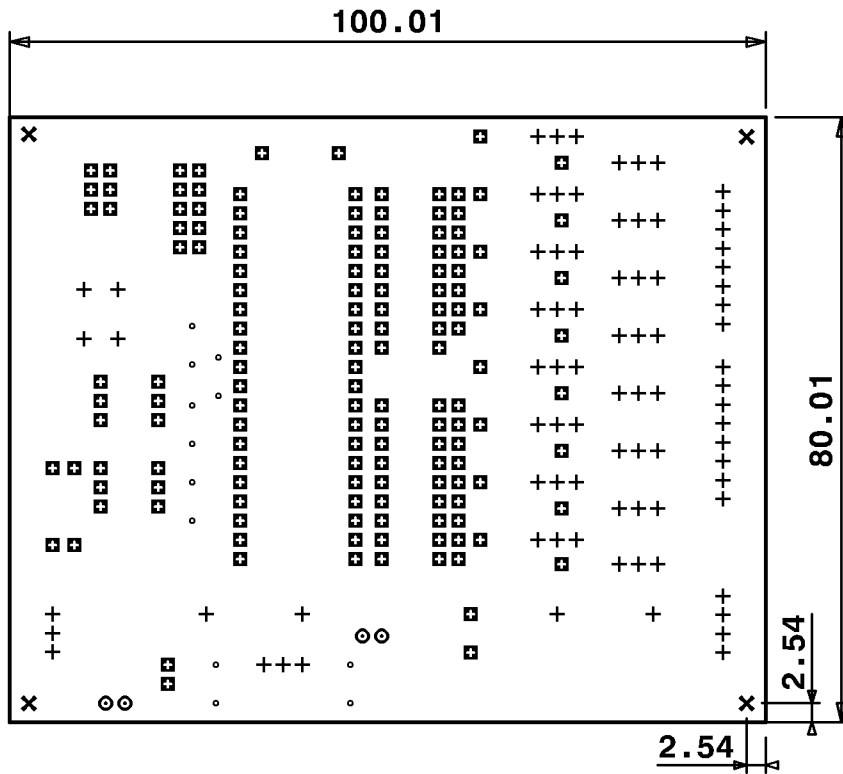
Drill Report : Layer E516969-60
